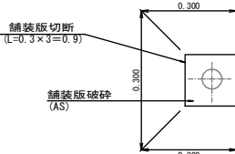
舗装破碎 S=1:20
